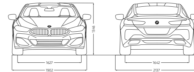
M850i xDrive
