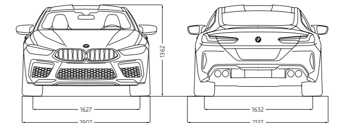
M8 Competition
