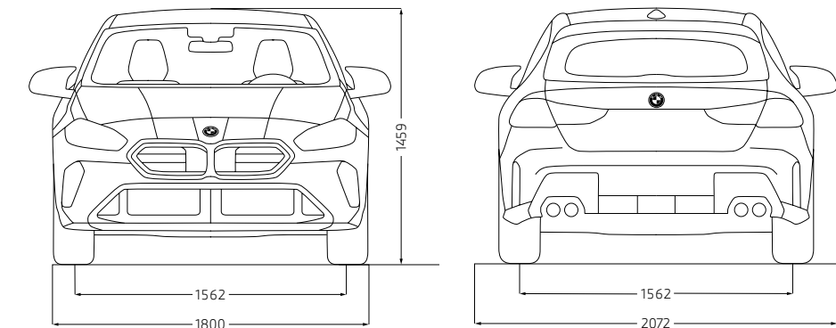
M135 xDrive
